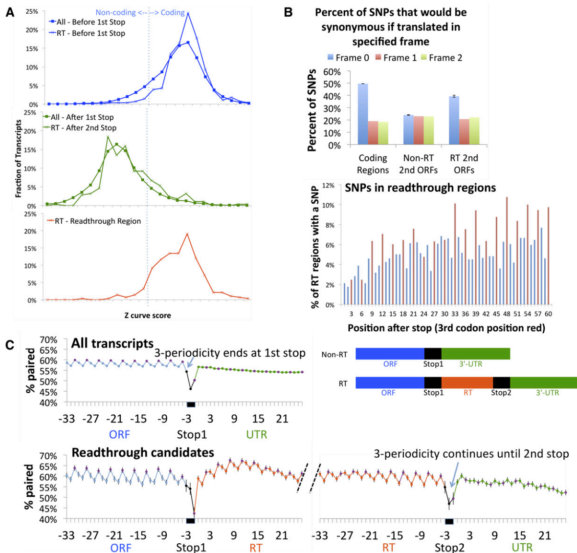
Figure 4. Single-species evidence of readthrough region translation. (A) D. melanogaster sequence composition of readthrough regions as measured by the Z curve statistic ( x -axis) suggests they are protein-coding (positive scores). (Top panel) Coding regions before the first stop for both readthrough candidates (crosses) and non-readthrough transcripts (squares) show positive Z curve scores typical of protein-coding regions. (Middle panel) Non-coding regions after the second stop for readthrough candidates (crosses) and after the first stop for typical transcripts (squares) show negative Z curve scores typical of non-coding regions. (Bottom panel) Readthrough regions show positive scores typical of protein-coding regions, providing single-species evidence that most readthrough regions are protein-coding. Evaluated regions in all panels were selected to match the length distribution of readthrough regions. (B) Single nucleotide polymorphisms (SNPs) show a strong bias to result in synonymous codon substitutions in readthrough regions (top right) and coding regions (top left), but no bias is seen in second ORFs downstream from non-readthrough stop codons (top middle), providing evidence that readthrough regions are under protein-coding selection within the D. melanogaster population. For each type of region we show the fraction of SNPs that would be synonymous if translated in each of three frames, with frame 0 matching the translated frame of the coding region of the gene. Error bars show the Standard Error of the Mean (SEM). As most third codon positions result in synonymous substitutions, the exclusion of non-synonymous substitutions is also visible as a periodicity in the fraction of readthrough candidates that have an SNP at each position of the second ORF (bottom panel), with third-codon-position SNPs (red) more prevalent than first or second-codon position SNPs (blue). This plot also shows an overall decrease in the number of SNPs near the readthrough stop codon, likely due to additional signals involved in regulating readthrough, such as RNA structures, encoded within the protein-coding signal. (C) Periodic base-pairing frequency in readthrough regions (red) matches that of known coding regions (blue) but is different from that of UTRs (green). Fraction of transcripts for which a given nucleotide is paired in predicted RNA secondary structures ( y -axis) at each position relative to a stop codon ( x -axis). Third codon positions (purple) are paired more frequently than first or second positions, and stop codons (positions -3 , -2 , and -1 ) show decreased pairing, as previously observed computationally in humans and experimentally in yeast (top panel). Transition from periodic to non-periodic pairing happens at the second stop codon for readthrough candidates (bottom panel). Signal is averaged over five codon positions (see Methods), with raw data shown in Supplemental Figure S2. Error bars show the Standard Error of the Mean (SEM).
